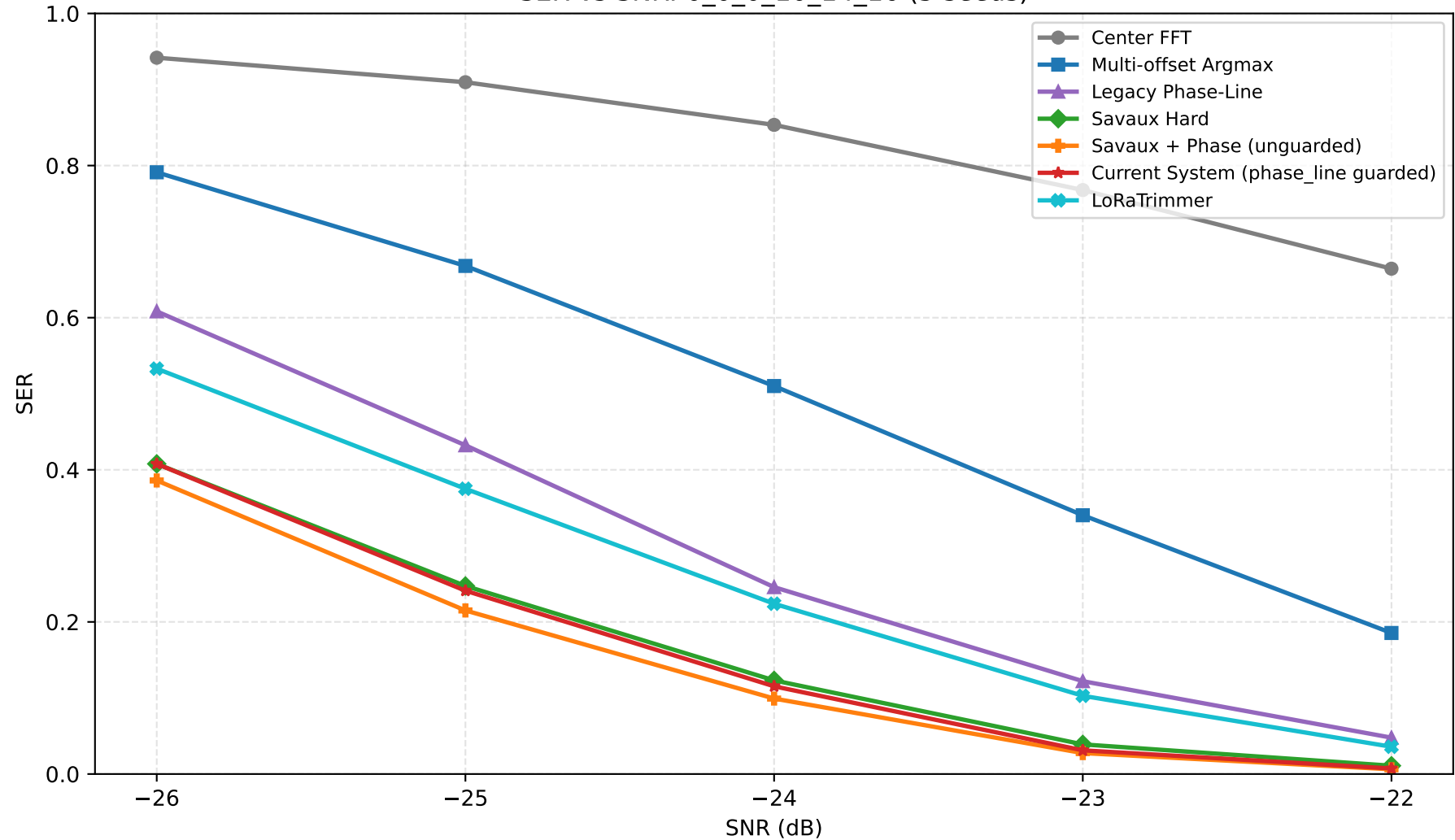
SER vs SNR: 0_0_0_10_14_16 (5 seeds)
